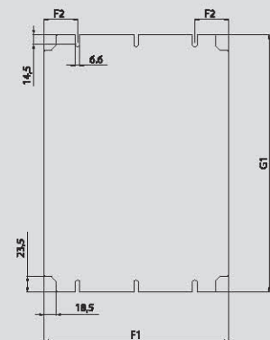
安装板细节图/Mounting Plate Detail Drawing
